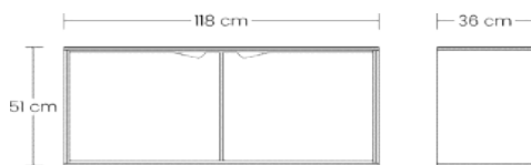
Model 5-402
