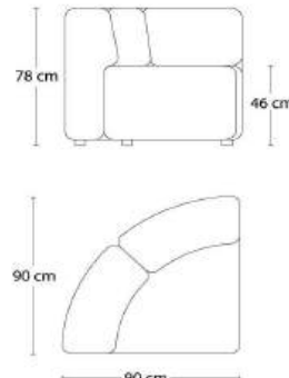
Model 3-6505
