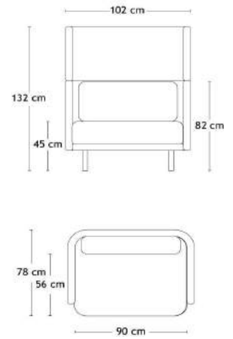
Model 3-6703
