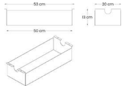
Model 9-7421
