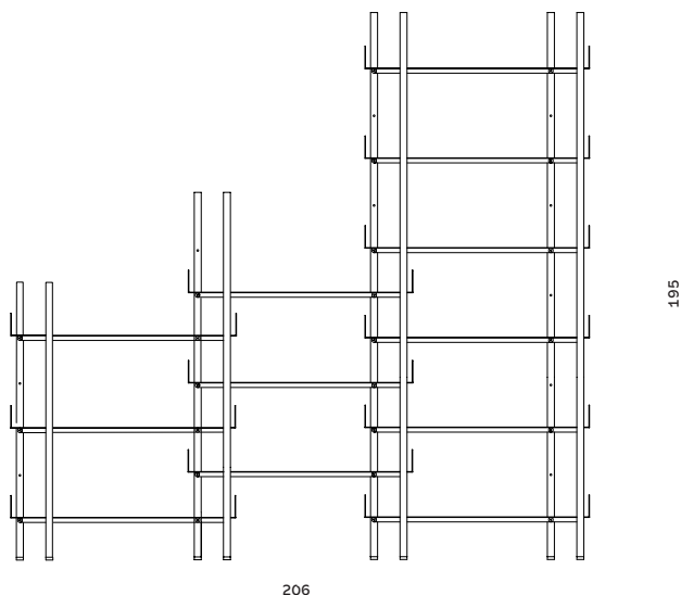
1 PKG LOW LEGS 32000031 / 32000026 1 PKG MEDIUM LEGS 32000030 / 32000025 2 PKG EXTRA HIGH LEGS 32000041 / 32000040 12 PCS SHELVES 32000032 / 32000027
