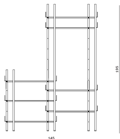
1 PKG LOW LEGS 32000031 / 32000026 2 PKG EXTRA HIGH LEGS 32000041 / 32000040 7 PCS SHELVES 32000032 / 32000027
