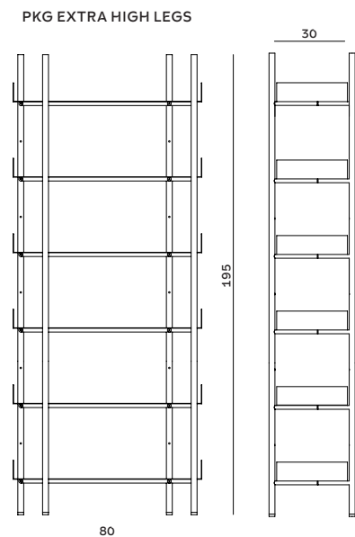
2 PKG EXTRA HIGH LEGS 6 PCS SHELVES
