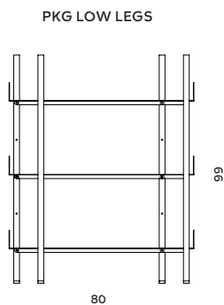
2 PKG LOW LEGS 3 PCS SHELVES
