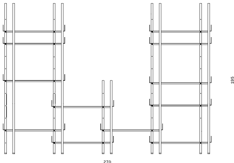
1 PKG LOW LEGS 32000031 / 32000026 4 PKG EXTRA HIGH LEGS 32000041 / 32000040 12 PCS SHELVES 32000032 / 32000027
