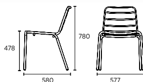
VG8087-02 Vega Aluminium Chair 4,3kg
