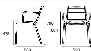
VG8086-04C Vega Padded Sling Armchair 3,1kg
