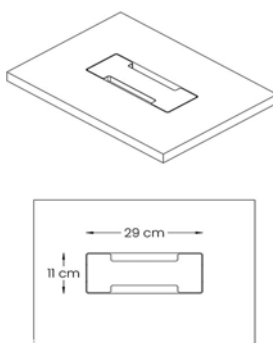
Model 0-2115- Drop-in Cover
